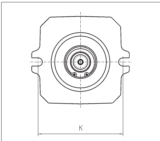
2-Loch Flansch
